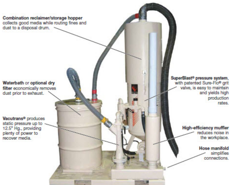
Blast-N-Vac-Features
